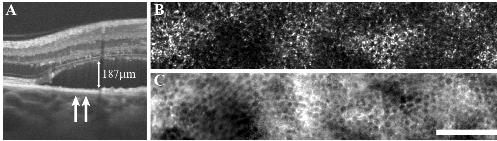
Fig. 12. RPE images collected in a patient DW_1188 with central serous retinopathy. The SD-OCT image in panel A shows the 187 \mu\text{m} thick fluid collection that separates the retina from the RPE (below). En face AOSLO images of the area between the white arrows in A show RPE morphology in confocal mode (B), as well as in dark-field mode (C) at this location approximately 6^\circ superior to fixation. The scale bar is 100 \mu\text{m} across.
