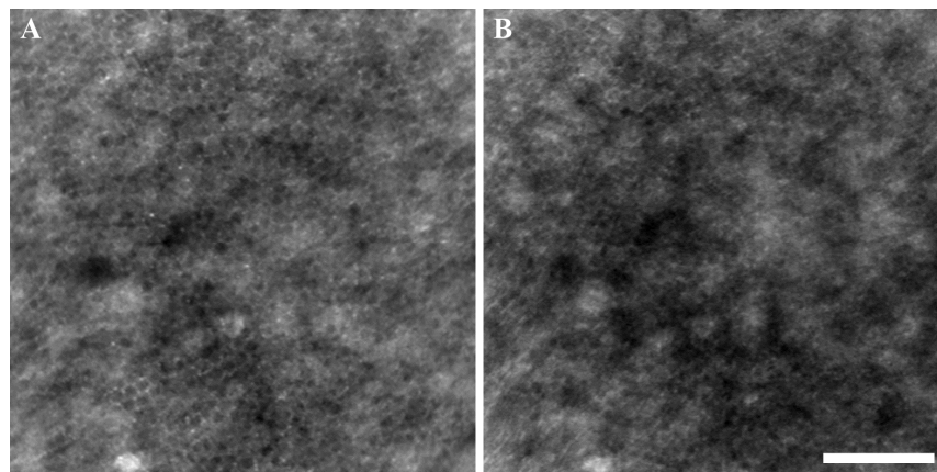
Fig. 9. Dark-field AOSLO images of the RPE mosaic at the center of fixation of volunteer JC_0616, using a 16 ADD diameter pinhole, 1 ADD thick filament and 790 nm (A) and 680nm (B) light. The scale bar is 100 \mu\text{m} across.
