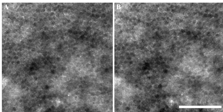
Fig. 7. Dark-field AOSLO images of the RPE mosaic at the center of fixation of volunteer JC_0616 collected using a 16 ADD diameter pinhole and either 1 (A) or 3 ADD thick filament (B). The scale bar is 100 \mu\text{m} across.
