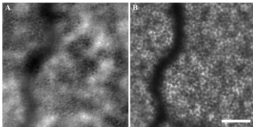
Fig. 11. Comparison of autofluorescence to dark-field RPE imaging in AD_1025 at 3^\circ superior and 9^\circ temporal from fixation. A) dark-field image, B) autofluorescence images collected using 565 nm excitation and 625 \pm 45 nm emission. The scale bar is 100 \mu\text{m} across.
