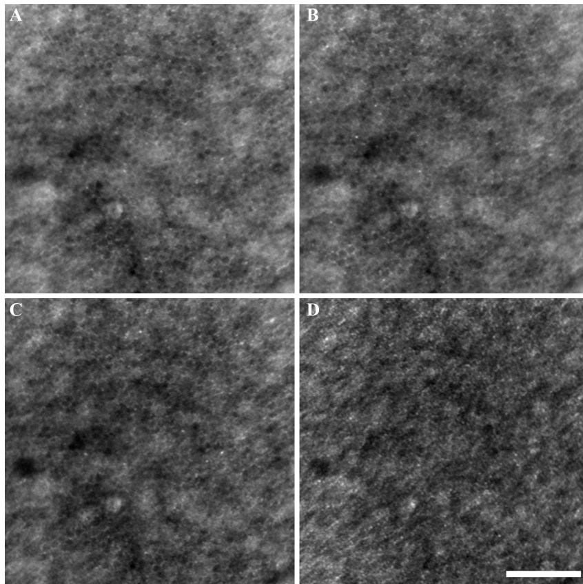
Fig. 6. Dark-field AOSLO images of the RPE mosaic at the center of fixation in volunteer JC_0616 collected using a 1 ADD thick filament and different pinhole diameters: A) 16, B) 12, C) 8 and D) 4 ADDs. The scale bar is 100 \mu\text{m} across.
