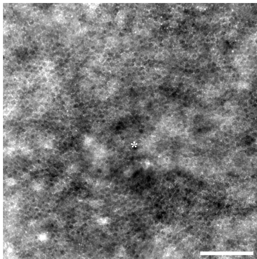
Fig. 13. AOSLO dark-field view from the fovea of volunteer JC_0616, with '*' denoting the point of maximum cone density. The scale bar is 100 \mu\text{m} across.
