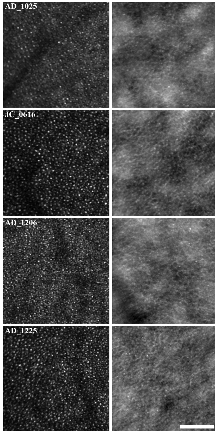
Fig. 3. AOSLO confocal (left) and dark-field (right) retinal images in four different subjects, all collected at 10° temporal to fixation. The confocal images show the cone and rod photoreceptor mosaic, while the dark-field images show the hexagonal RPE cell mosaic with significant cross-talk from the photoreceptor mosaic. The scale bar is 100 \mu\text{m} across.
