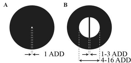
Fig. 1. AOSLO image plane apertures in front of the detector: A) traditional confocal pinhole, approximately one Airy disk diameter (ADD), and B) large pinhole with centered filament.
