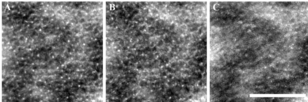
Fig. 10. Effect of pupil apodization on image quality and contrast at 10^\circ temporal to fixation in volunteer JC_0616 using 790 nm illumination, 16 ADD pinhole, 1 ADD filament (A) and with a centered 3 mm diameter circular block in the imaging (B) or the illumination paths (C). The scale bar is 100 \mu\text{m} across.
