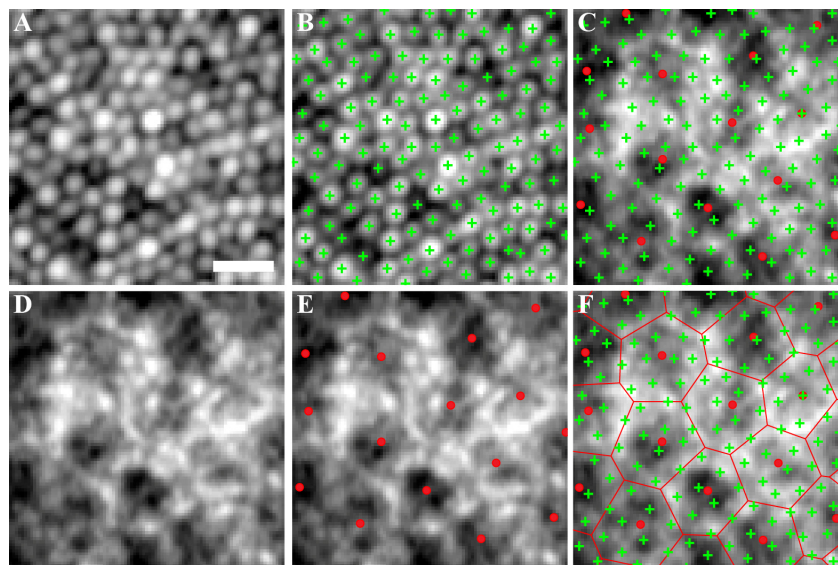
Fig. 5. Confocal (photoreceptor) and dark-field (RPE) images collected simultaneously (subject JC_0616) at approximately 0.8^\circ from fixation. Panels A-B and C-F show cones recorded with 1 ADD pinhole and dark-field recorded with a 16 ADD pinhole and 1 ADD filament, respectively. Panels B and E show the cone and RPE cell centers marked with crosses and circles superimposed to the images in A and D, respectively. Panel C shows the dark-field image with cone centers and RPE centers superimposed, while panel F adds the cell borders, determined as Voronoi cells derived from the estimated cell centers. The scale bar is 10 \mu\text{m} across.
