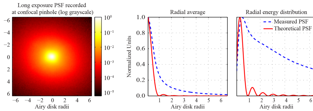
Fig. 8. Time-averaged retinal point-spread function (PSF) recorded from research volunteer JC_0616 (left), focused on the photoreceptor layer (logarithmic color scale). The central and right panels show the radial average and integral, respectively, compared to that of a single retinal layer theoretical PSF (red solid lines).
