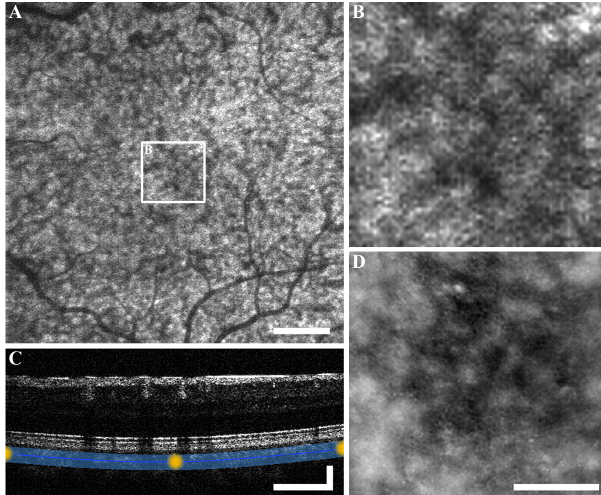
Fig. 4. Comparison of SD-OCT data and an AOSLO dark-field image (subject AD_1025). The en face view shown in B was created by coarsely segmenting the SD-OCT signal from the choroid over the area highlighted in panel A over the depth range indicated by the blue band. Panel D, shows the same retinal area as B as seen using AOSLO dark-field imaging. Scale bars are: A) 500 \mu\text{m} ; C) 500 \mu\text{m} horizontal and 100 \mu\text{m} vertical; B) & D) 100 \mu\text{m} .
